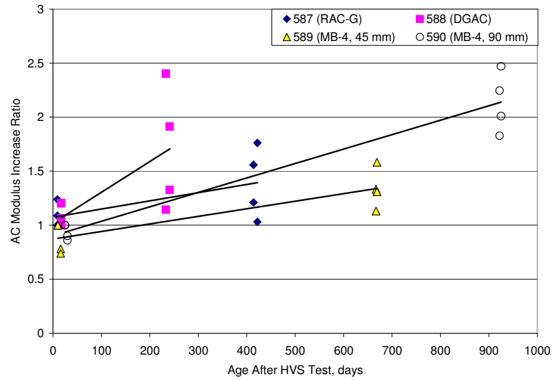
Figure 4.27: Normalized moduli versus age after HVS test.
