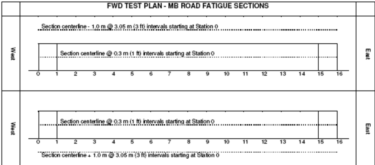
Figure 2.8: FWD test plans (test track and HVS trafficked section).
