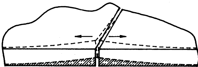
Figure 4.1. Edge and corner curling caused by daily temperature variation.
