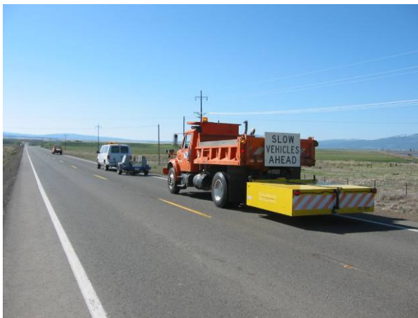
Example of a safe experimental section
