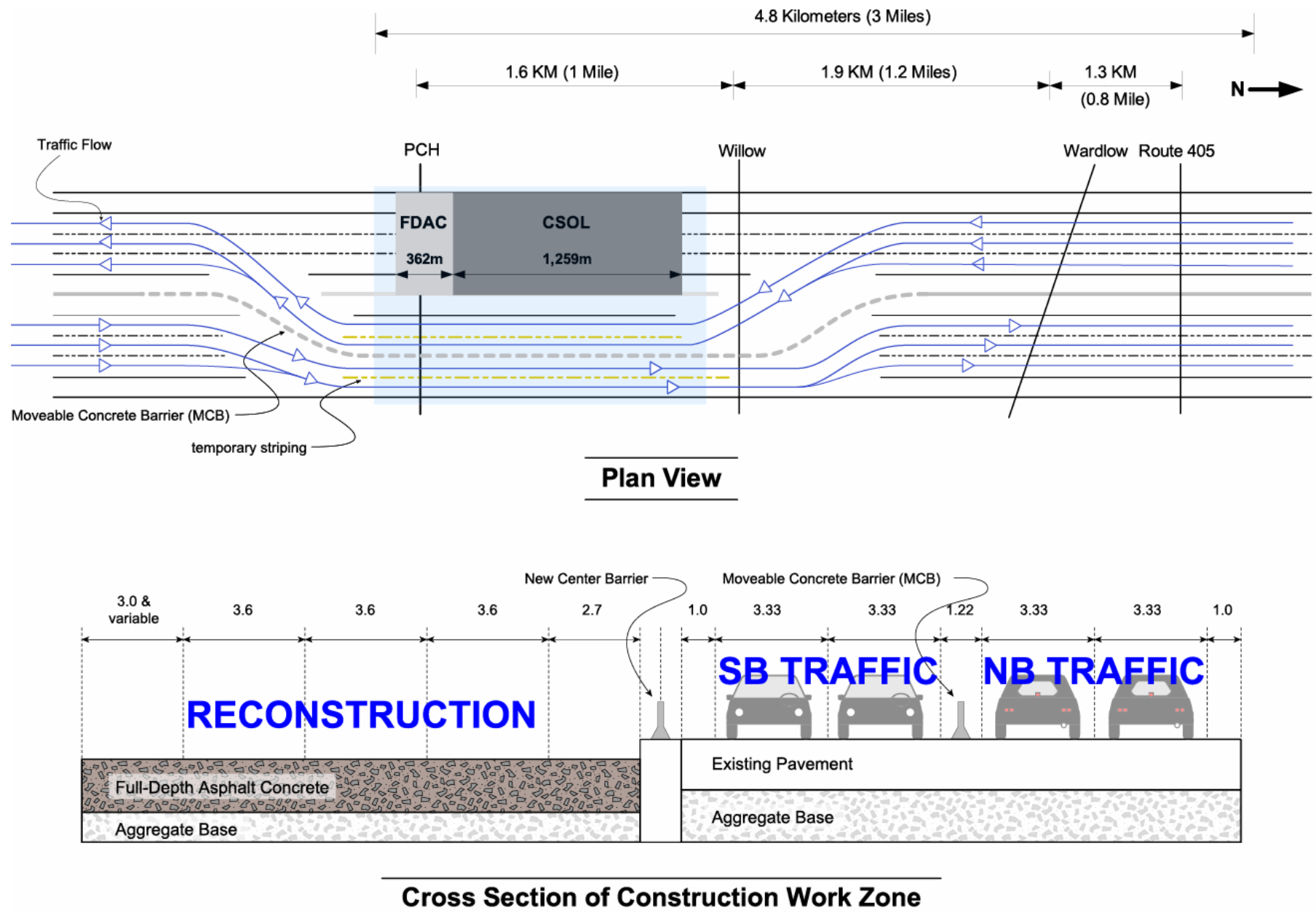
Figure 1. Lane closure tactics for the first 55-hour weekend closure at Pacific Coast Highway.
