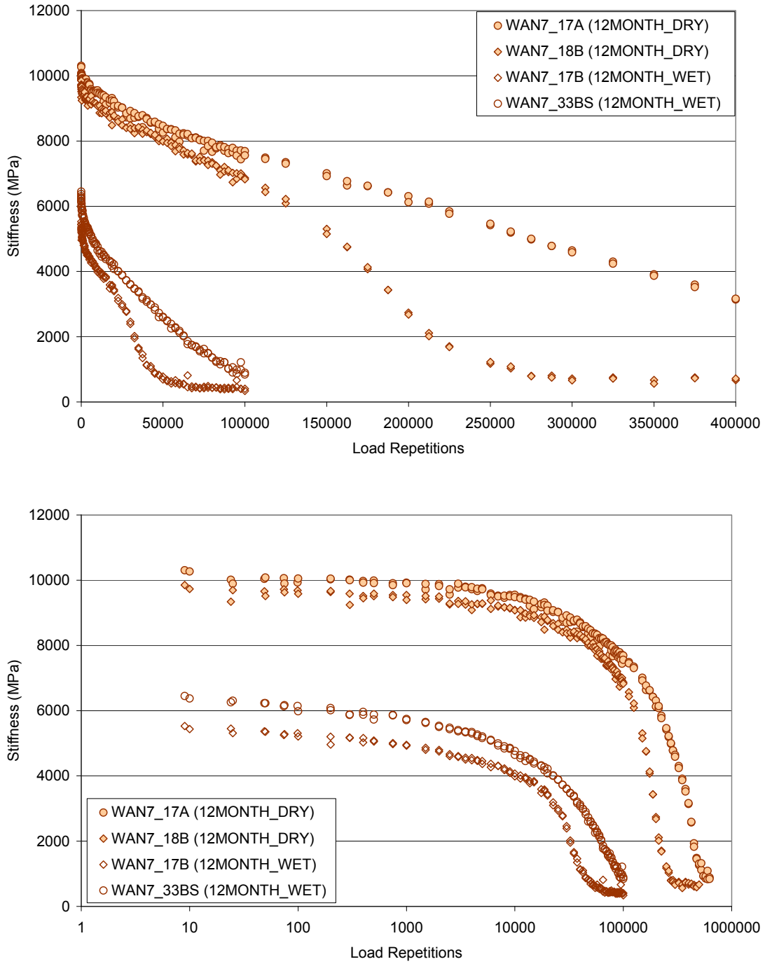
Figure H-4. Stiffness deterioration curves of mix AAN after twelve-month conditioning.
