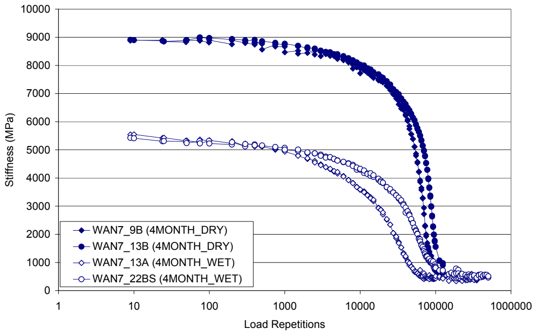
Figure H-2. Stiffness deterioration curves of mix AAN after four-month conditioning.
