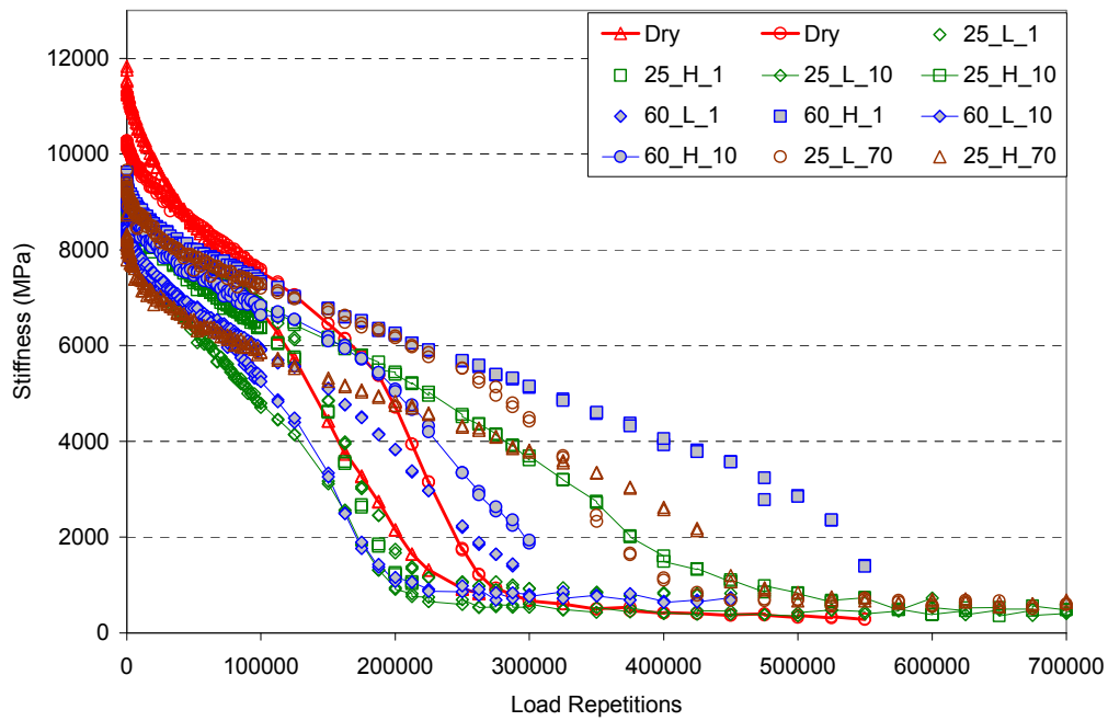
Figure 6-5. Stiffness deterioration curves of AAM.
