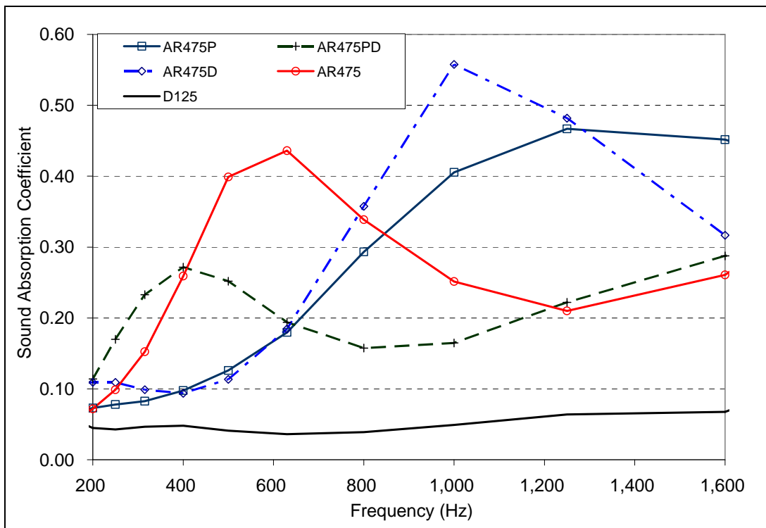
Figure 5.35: Spectra of sound absorption coefficients of mixes with 4.75 mm NMAS and various gradations and air-void contents.
