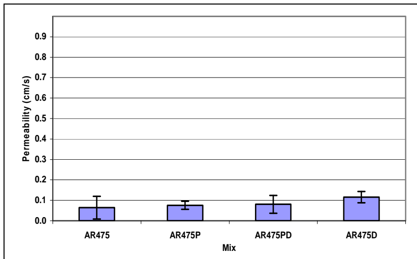
Figure 4.20: Comparison of effect of better compaction on permeability (4.75 mm mixes).
