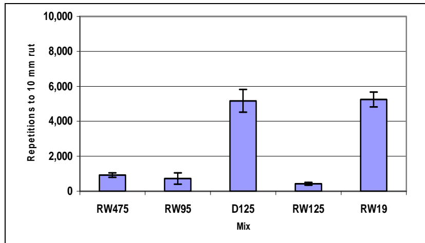
Figure 4.23: Comparison of effect of maximum aggregate size on moisture sensitivity.
