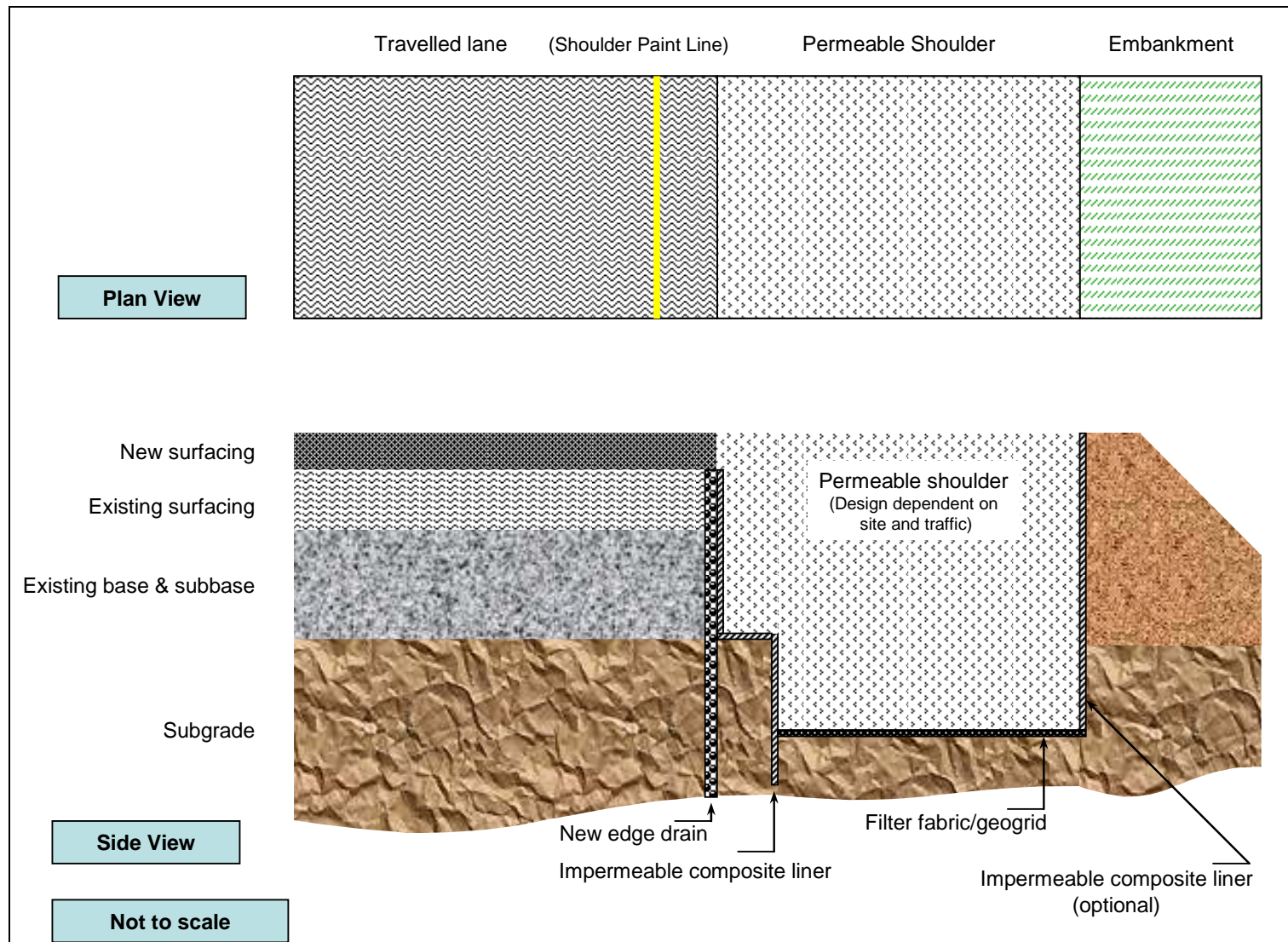
Figure 6.2: Example fully permeable pavement shoulder retrofit #2.
