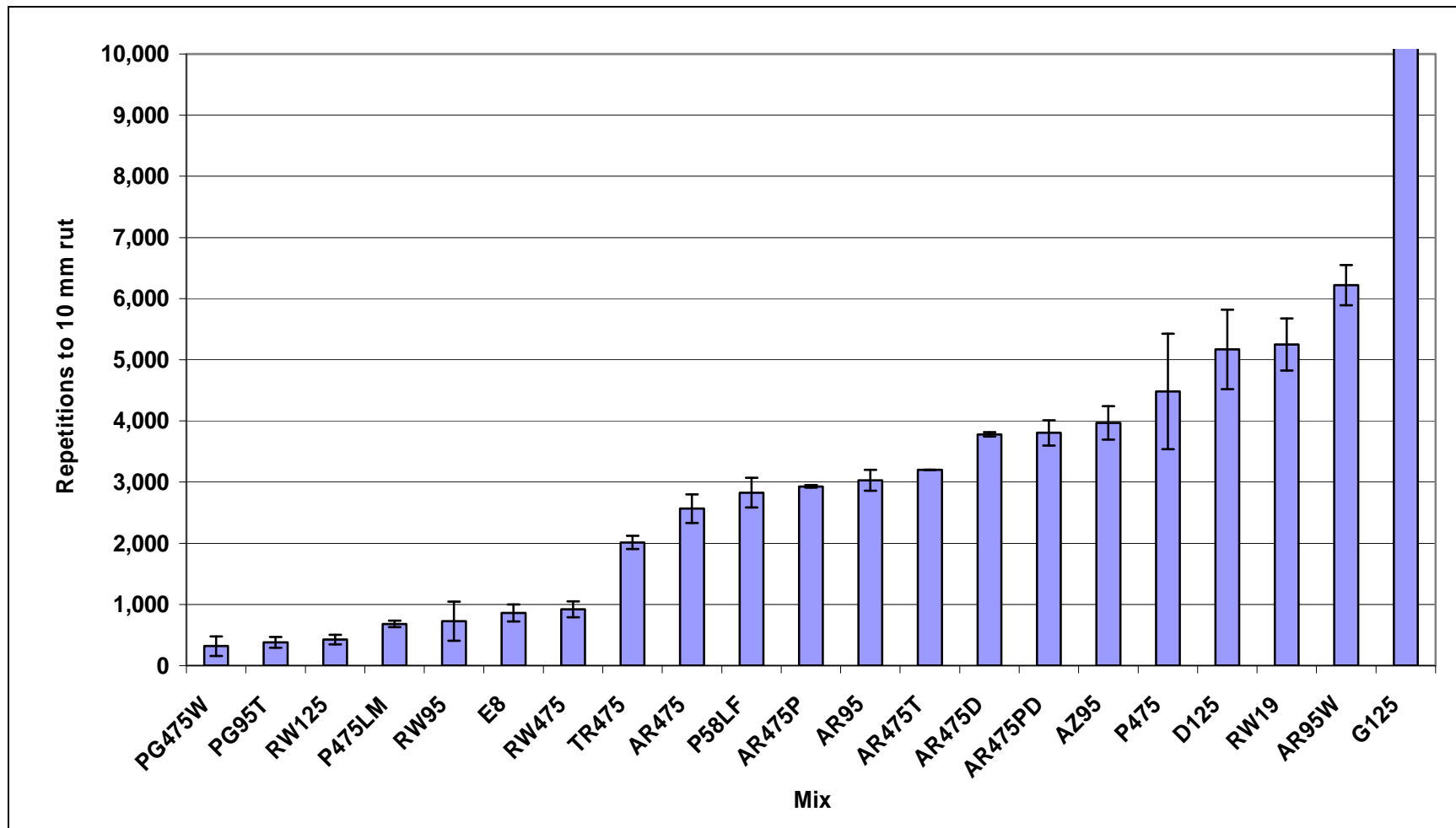
Figure 4.22: Summary plot of ranked HWT results for all mixes.
