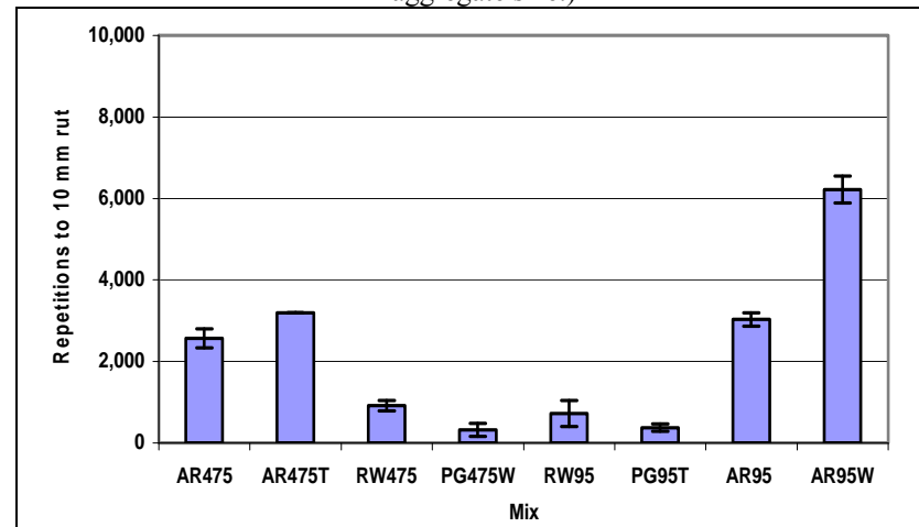
Figure 4.26: Comparison of effect of different aggregate types on moisture sensitivity.
