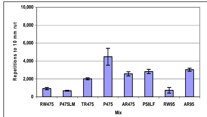
Figure 4.24: Comparison of effect of different binders on moisture sensitivity.
