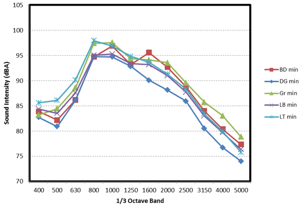
Figure 3.15: Comparison of OBSI spectral content of sections with different texture types, minimum of sections with aged texture. (Note: BD = burlap drag, DG = diamond ground, Gr = diamond grooved, LB = longitudinally broomed, LT = longitudinally tined.)
