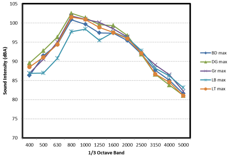
Figure 3.16: Comparison of OBSI spectral content of sections with different texture types, maximum of sections with aged texture. (Note: BD = burlap drag, DG = diamond ground, Gr = diamond grooved, LB = longitudinally broomed, LT = longitudinally tined.)
