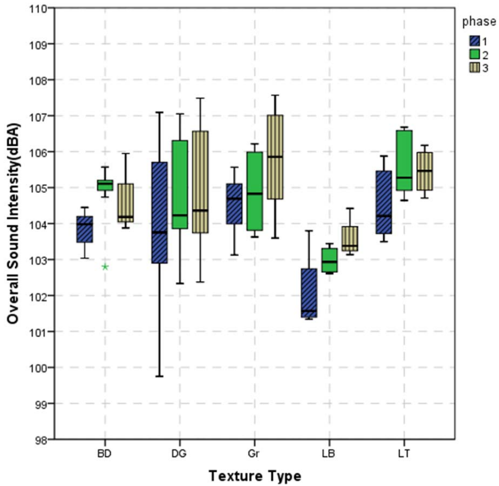
Figure 3.19: Box plots of OBSI results by texture type, all measurements from Years 1, 2, and 3, with aged condition. (Notes: BD = burlap drag, DG = diamond ground, Gr = diamond grooved, LB = longitudinally broomed, and LT = longitudinally tined.)
