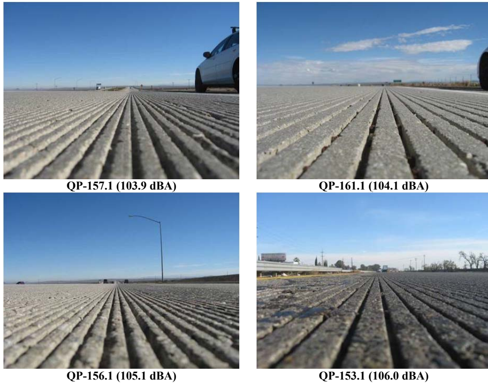
Figure 4.4: Example photographs of diamond-grooved surfaces and their OBSI levels.
