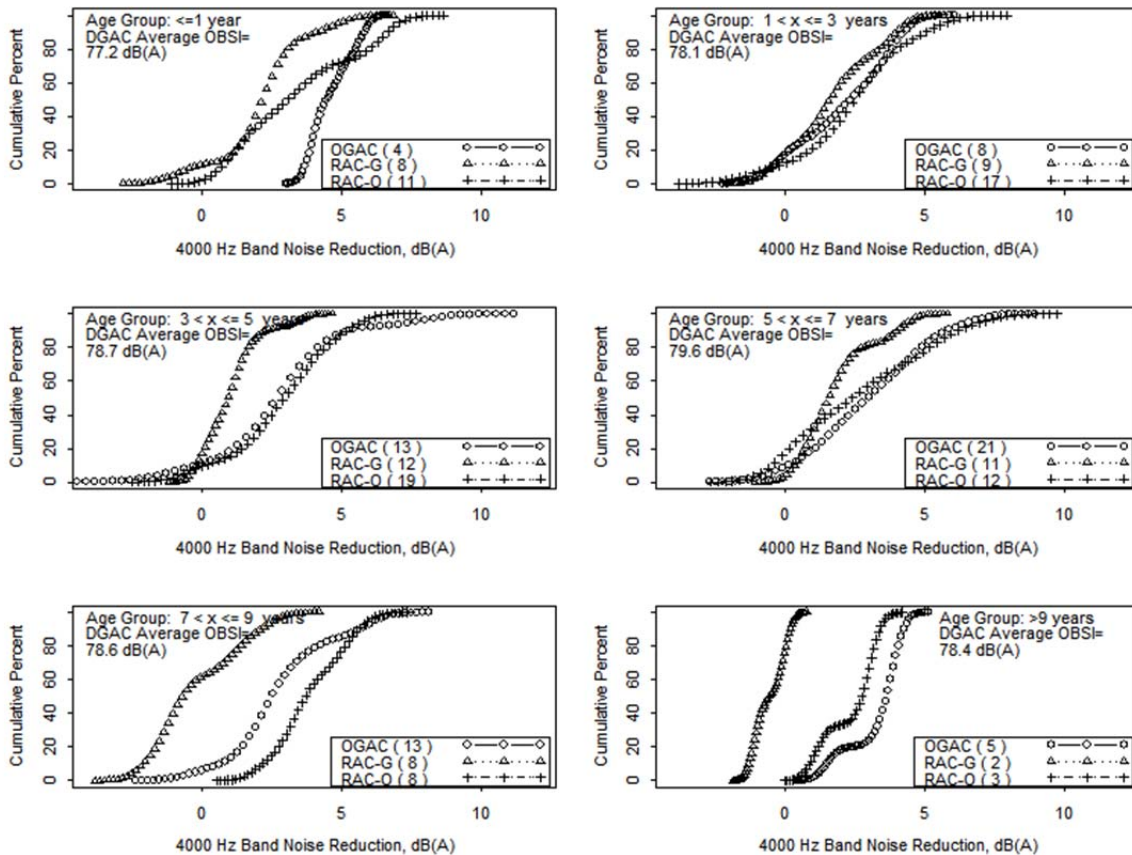
Figure A.27: Estimated cumulative distribution function of 4,000-Hz noise reduction of OGAC, RAC-O, and RAC-G mixes for different groups by pavement age.
