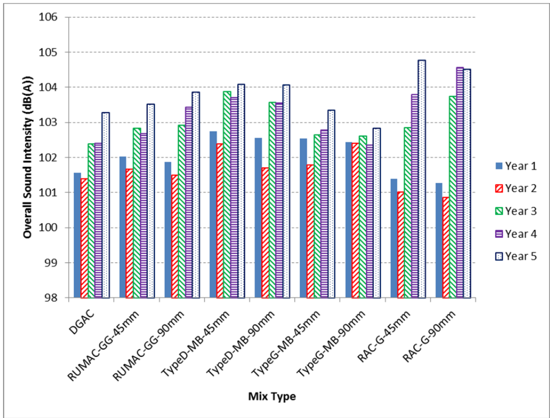
Figure A.30: Five-year overall OBSI values for Fresno 33 sections.
