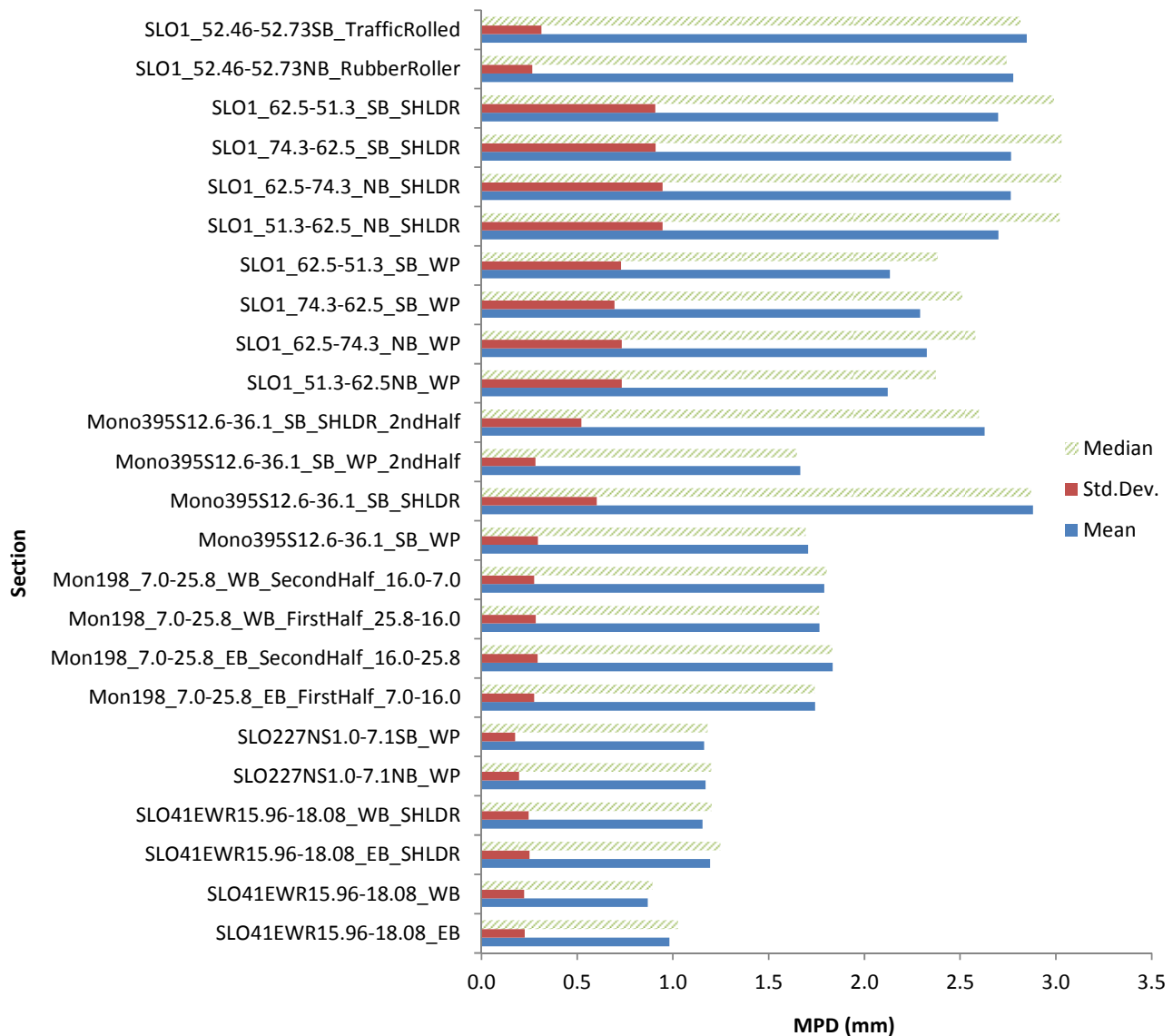
Figure 4.15: Median, mean, and standard deviation of MPD measured from IP for different Phase I sections. (Note: SHLDR is for outside of ETW; WP is for inside of ETW.)
