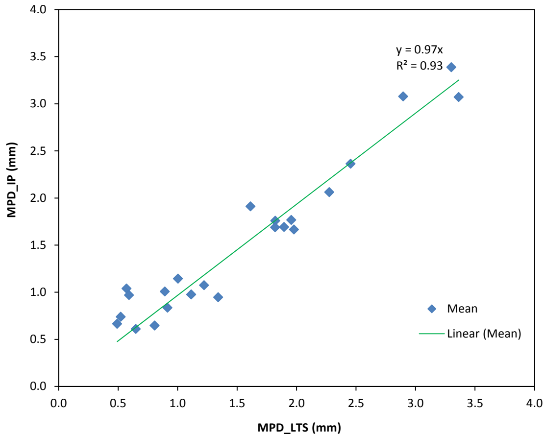
Figure 5.18: Correlation of macrotexture measurements with IP and LTS.
