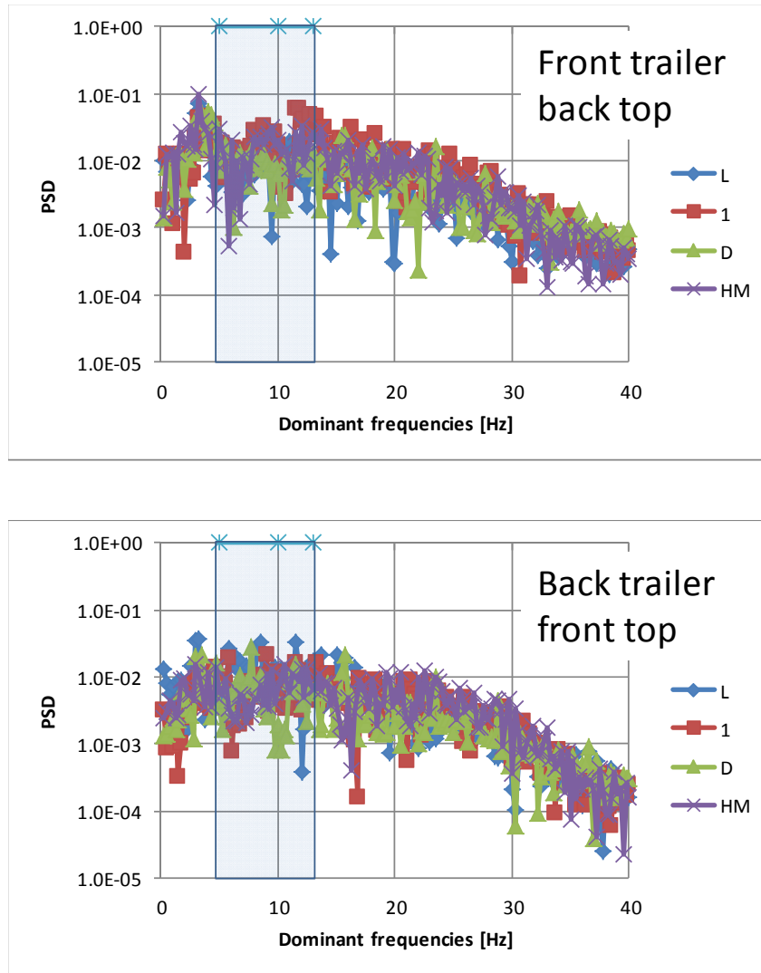
Figure 5.4: Comparison between dominant frequencies at two locations on trailers and tomato sensitivity frequencies that may result in fruit damage.
