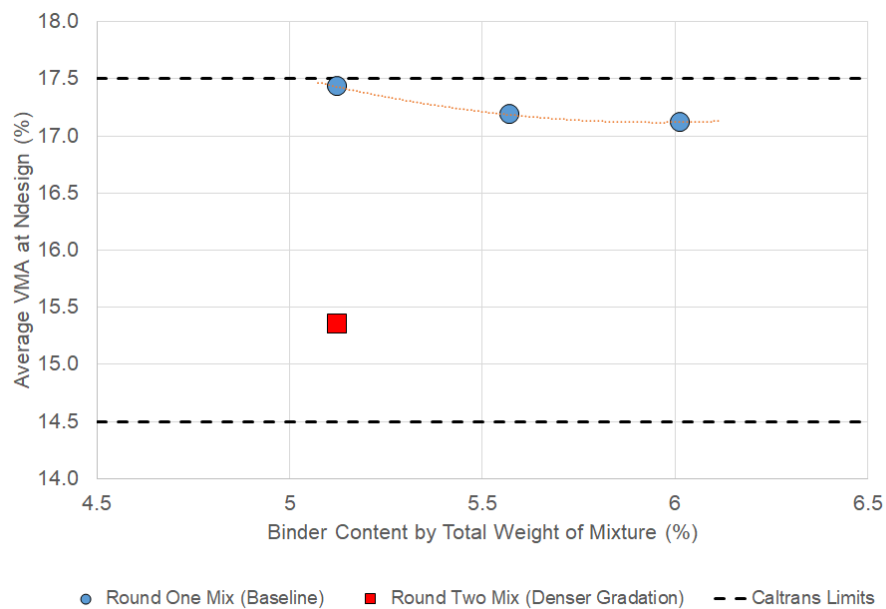
Figure 5.2: VMA at Ndesign gyrations for the Round One and Round Two mixes.
