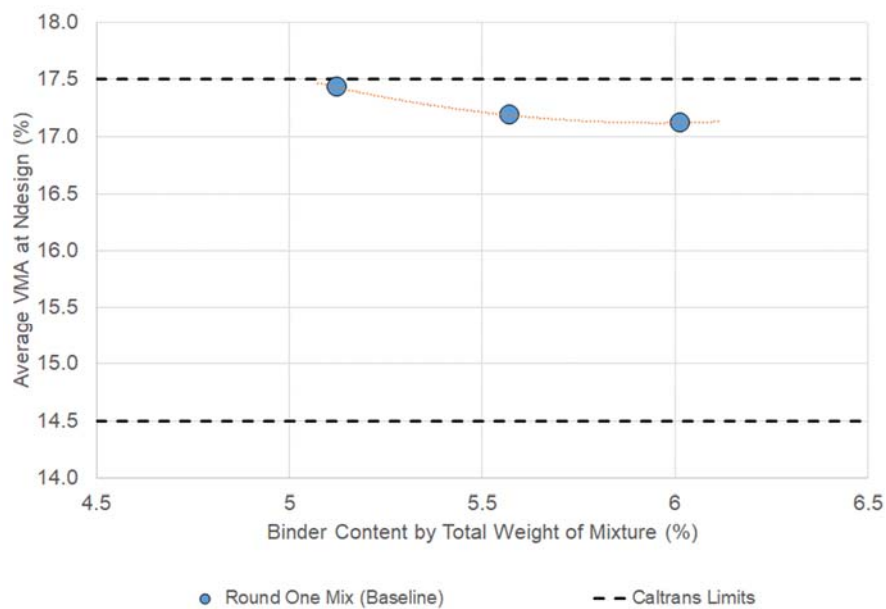
Figure 3.6: Variation of VMA at Ndesign gyrations with binder content.
