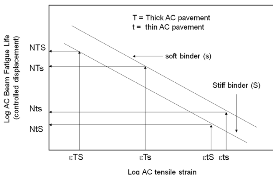
Figure 8.4: General rules of fatigue resistance and stiffness.
