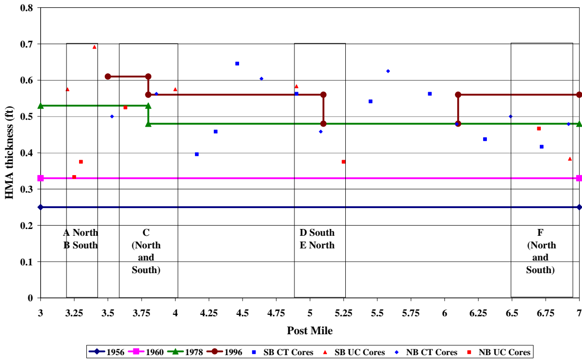
Figure 8: HMA core thicknesses (2007) by section, post mile, and construction history from as-builts.
