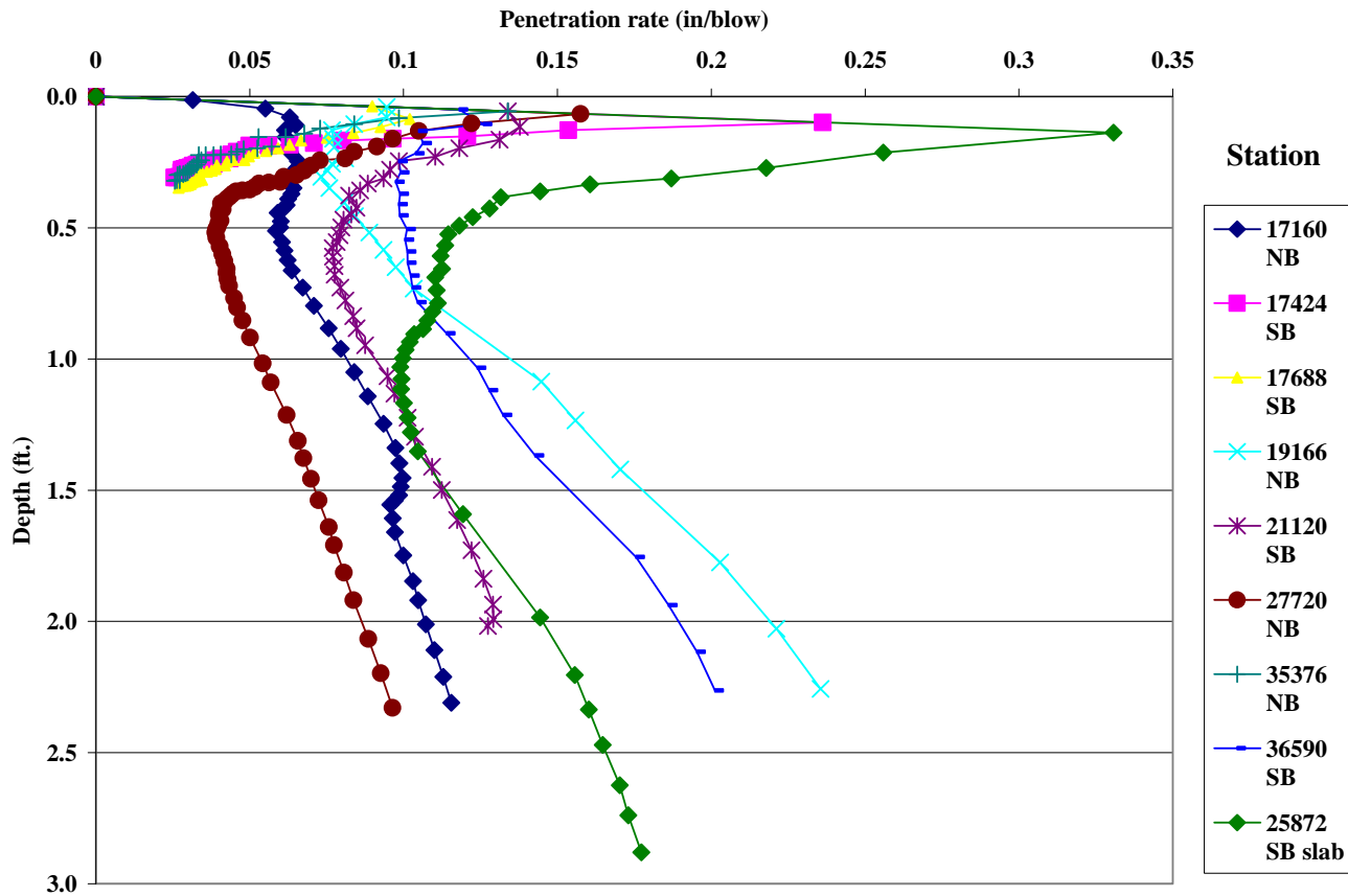
Figure 10: DCP locations and results. (Depth is depth below top of AB layer.)
