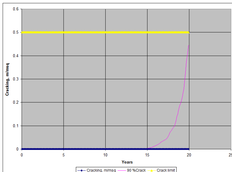
Figure A.7: Typical cracking-versus-age plot from CalME (Table 8, Design Option 2, PG 64-16 HMA mill and fill).
