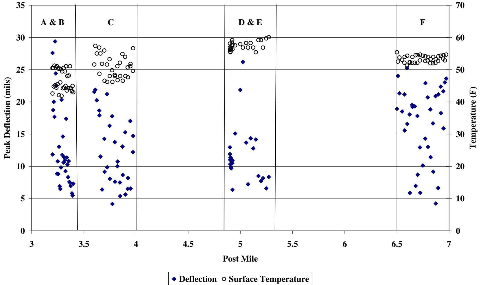
Figure A.3: FWD inner sensor (D1) peak deflection and surface temperature versus post mile.
