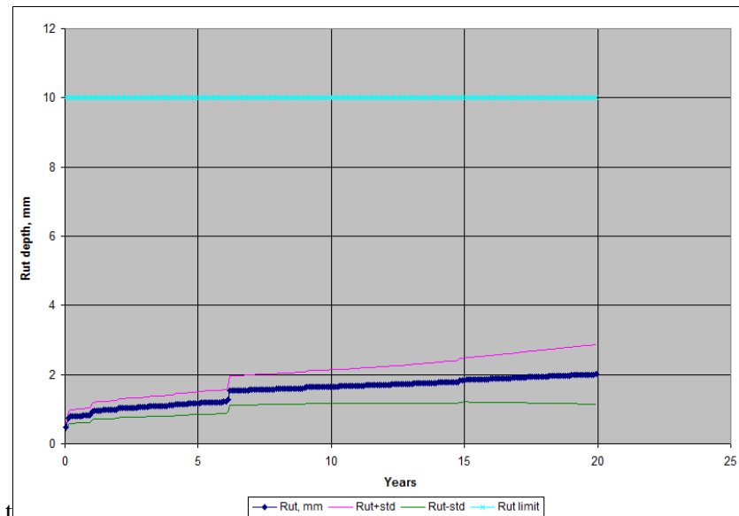
Figure A.6: Typical rutting-versus-age plot from CalME (Table 8, Design Option 2, PG 64-16 HMA mill and fill).
