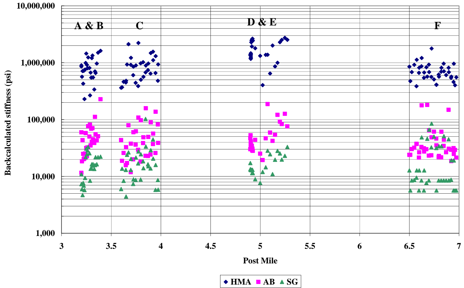
Figure A.5: Backcalculated layer stiffness (temperature adjusted to 68° F) versus post mile.
