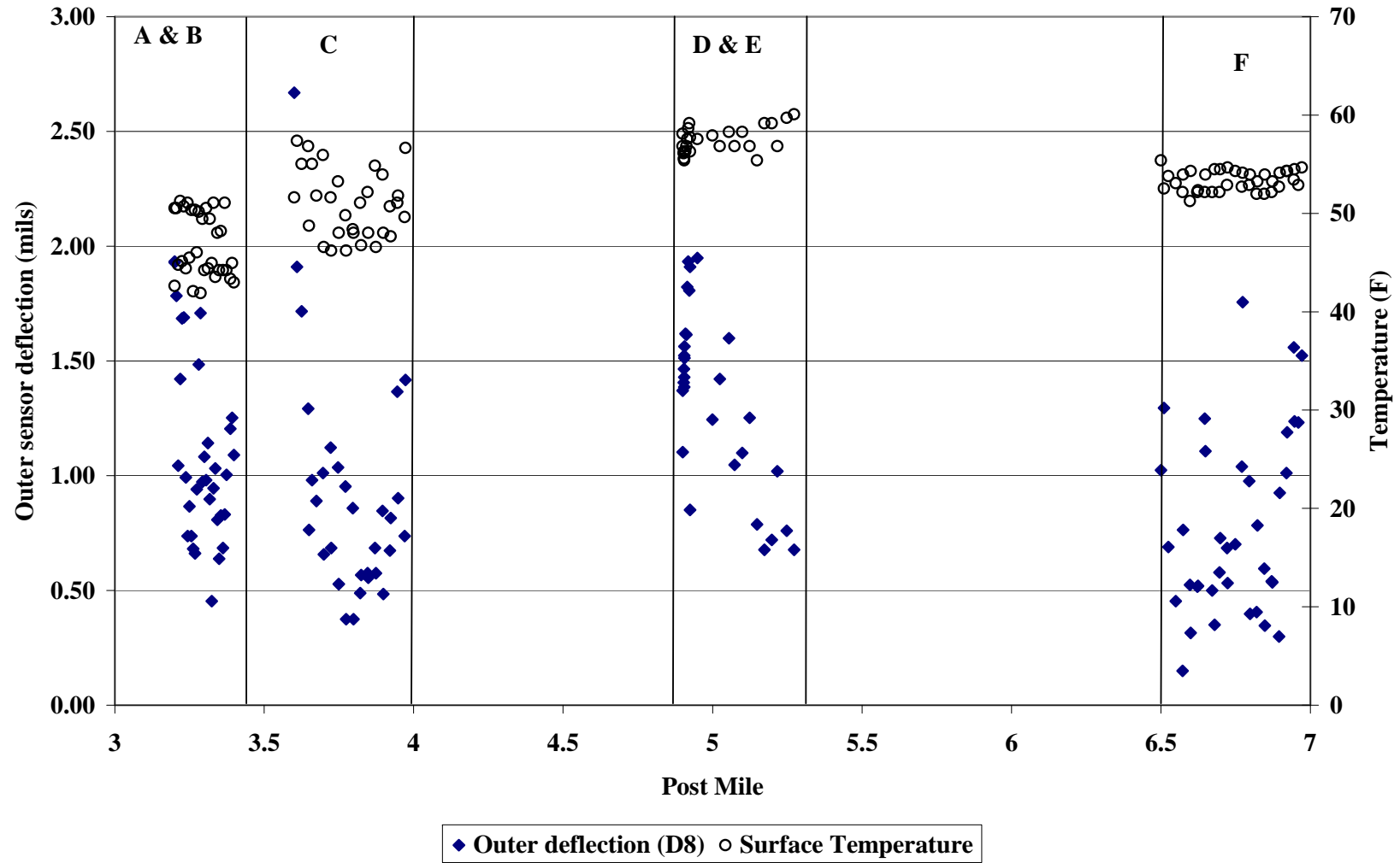
Figure A.4: FWD outer sensor (D8) peak deflection and surface temperature versus post mile.
