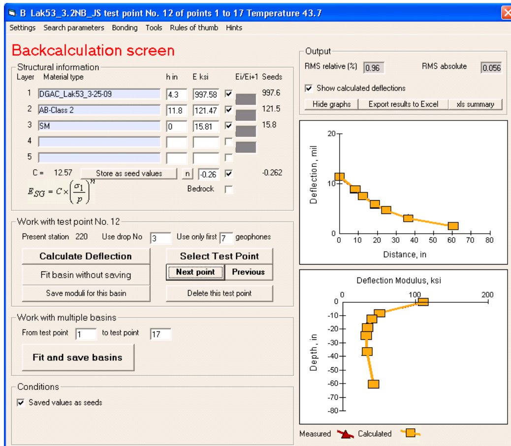
Figure 9: CalBack screen shot of the deflection bowl and corresponding deflection modulus at Test Point 12, Lake 53, PM 3.2 NB.
