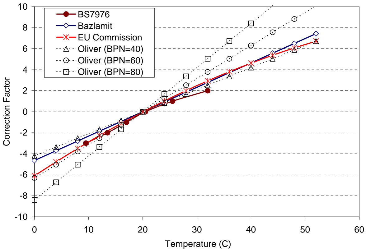
Figure 3.1: Various temperature correction factors for British Pendulum Numbers (1).
