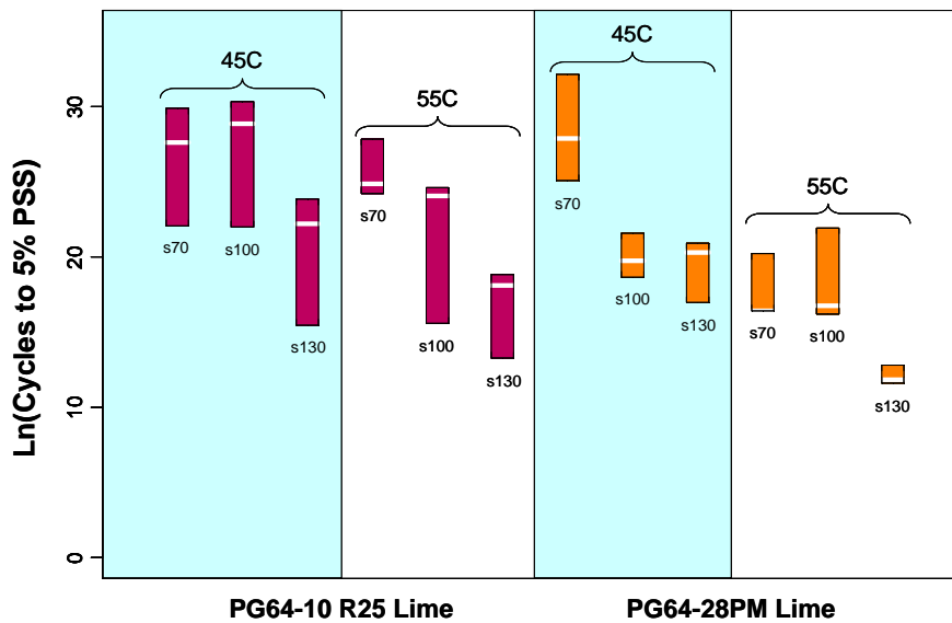
Figure A.8: \text{Ln}(G) at three shear stress levels and at 45°C and 55°C; Red Bluff Project (PG 64-28PM and PG 64-10 mixes).
