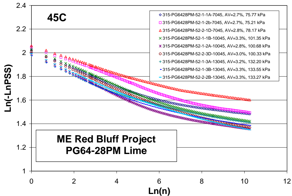
Figure A.4: Summary of shear test results at 45°C, \ln(\ln(\gamma_p)) versus \ln (load repetitions), PG 64-28PM mix (ME, Red Bluff Project, AC = 5.2% [by weight of aggregate plus lime], 1.2% lime, AV = 3.0%, LMLC).
