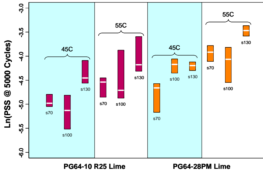
Figure A.7: \text{Ln}(\gamma_p \text{ at } 5,000 \text{ load repetitions}) at three shear stress levels and at 45°C and 55°C; Red Bluff Project (PG 64-28PM and PG 64-10 mixes).
