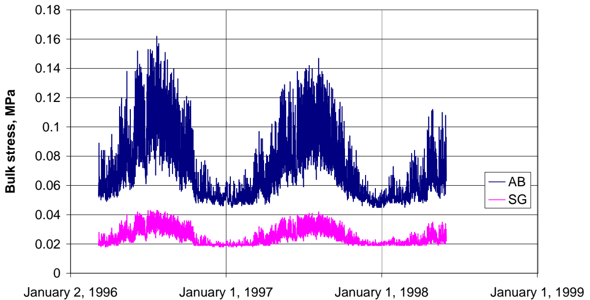
Figure 45. Bulk stress in aggregate base and in subgrade, 50 mm below the surface of the layers, Section 18, calculated using CalME.
