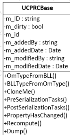
Figure 5.4: The Base Class, UCPRCBase .
