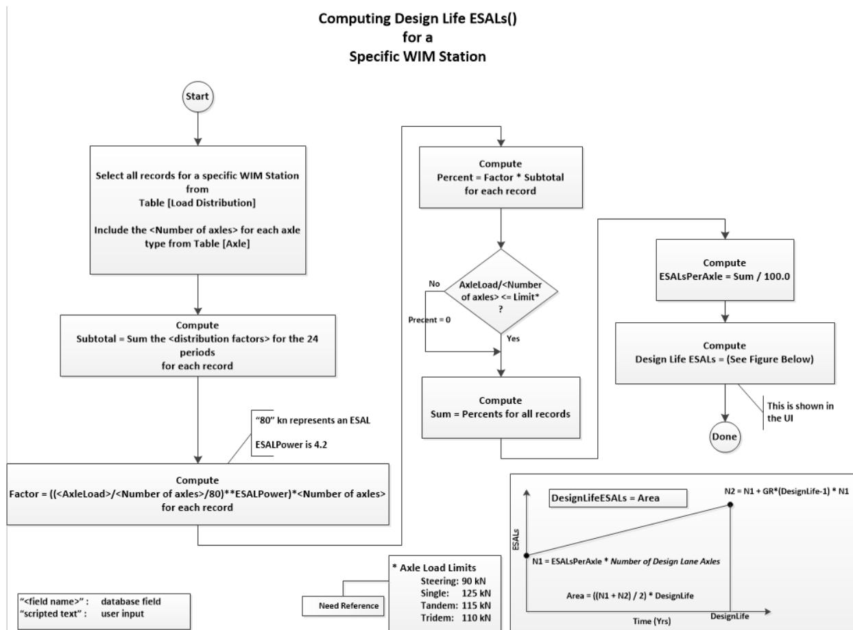
Figure 2.9: Flowchart for computing ESALs/yr.
