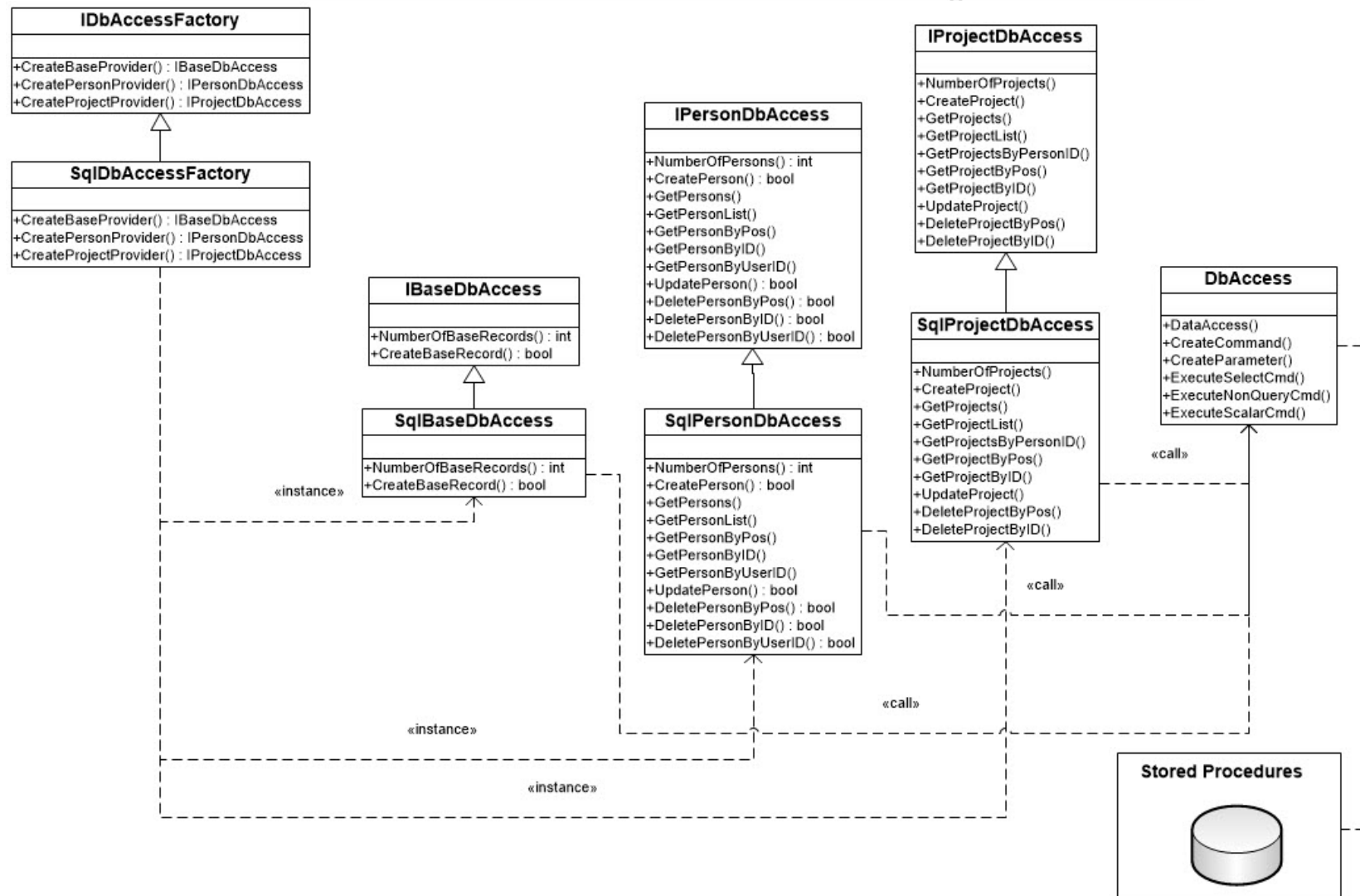
Figure 5.2: Factory Pattern implemented in DAL.
