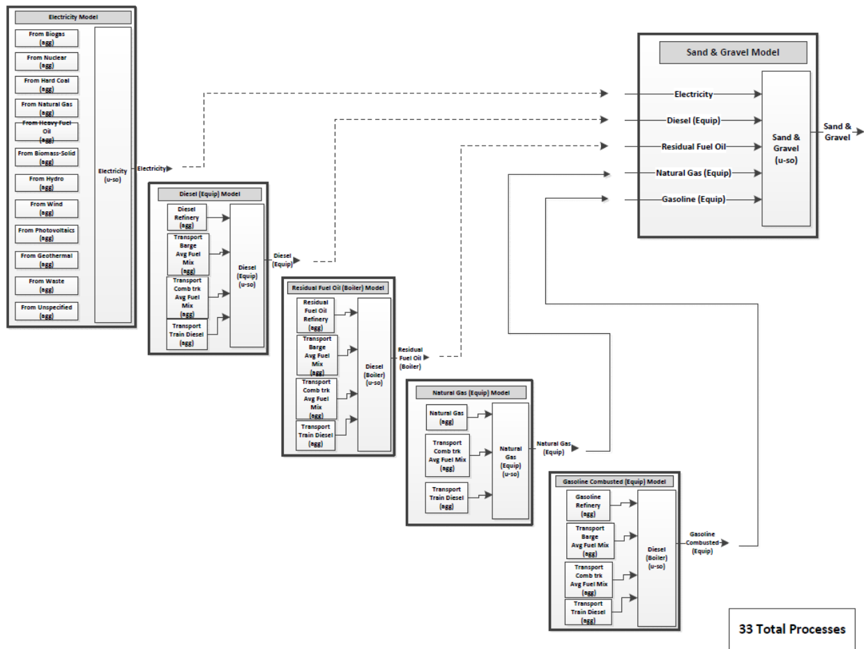
Figure A.8: Sand &amp; Gravel Process Model.
