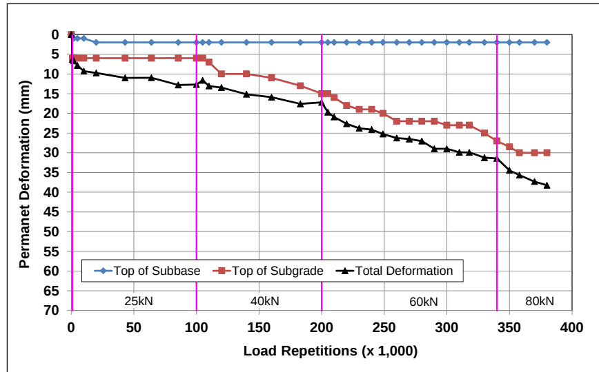
Figure 7.28: 679HC 950 mm: Permanent deformation in the underlying layers.
