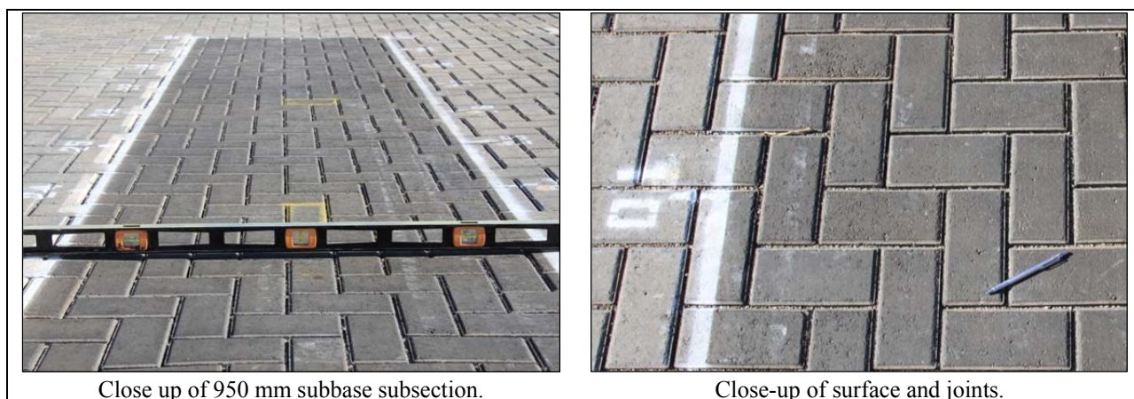
Figure 7.41: 680HC: Test section photographs.
