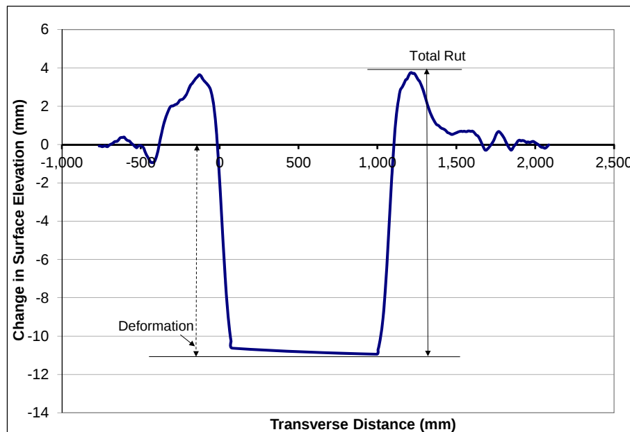
Figure 6.6: Illustration of maximum rut depth and deformation for a leveled profile. (For HVS test with 1 m wander)
