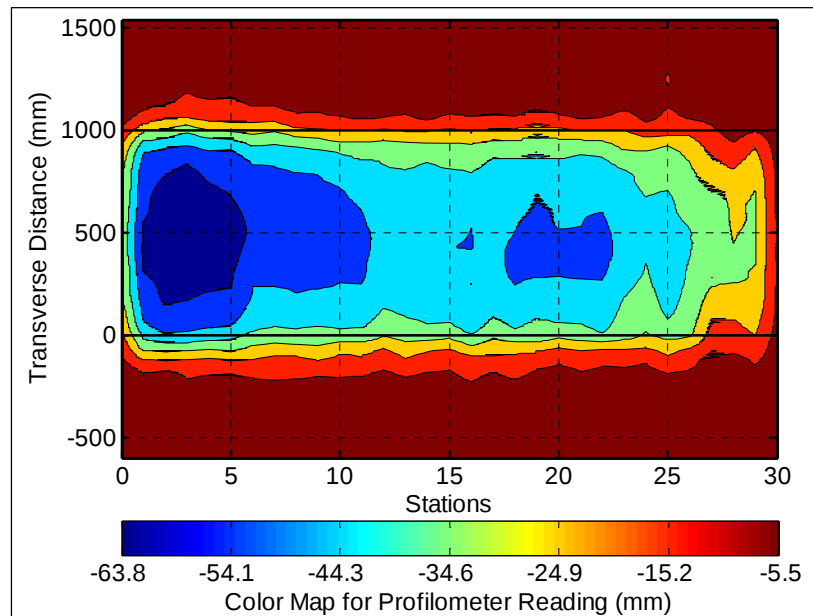
Figure 7.25: 679HC: Contour plots of permanent surface deformation (380,000 repetitions).
