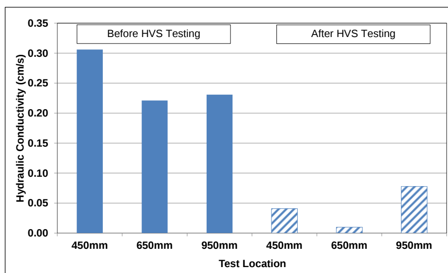
Figure 7.42: Surface permeability before and after HVS testing.
