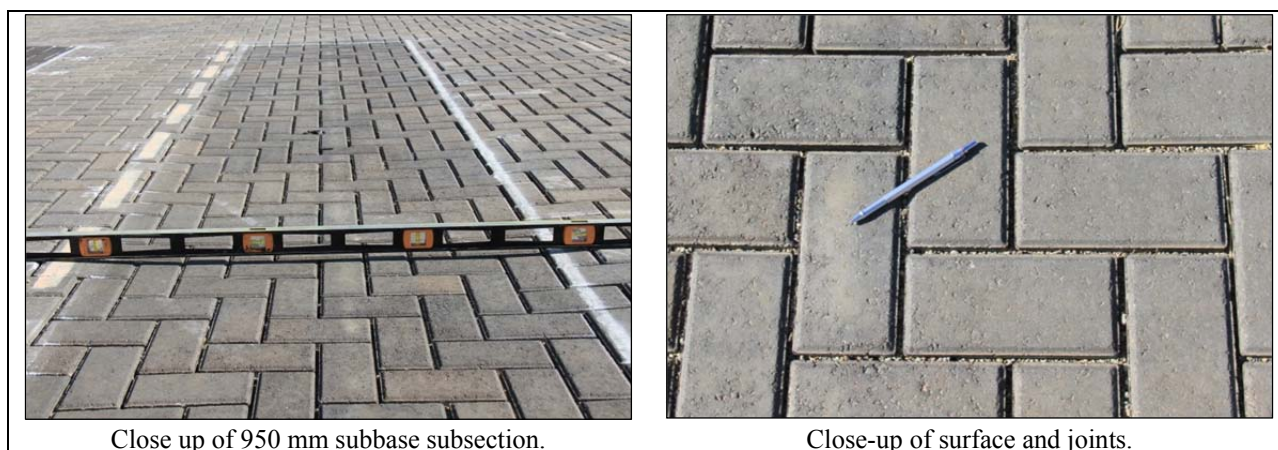
Figure 7.16: 678HC: Test section photographs.
