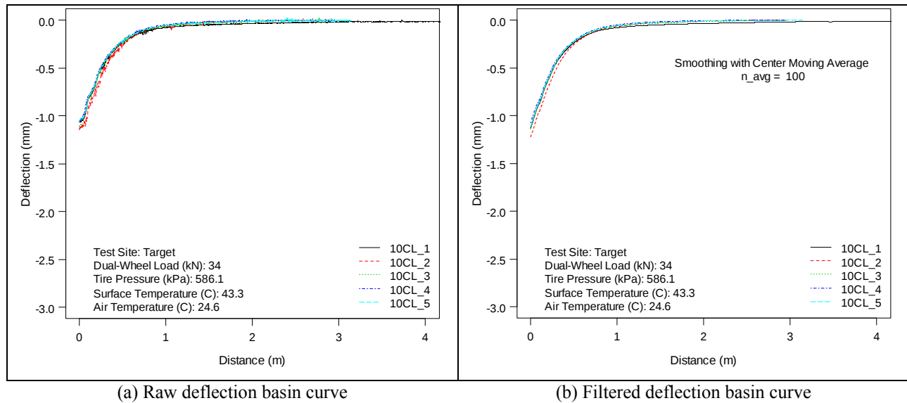
Figure 3.1: Raw and filtered deflection basin curves.
