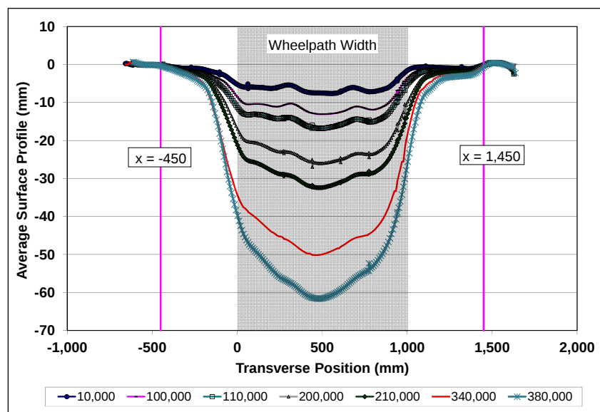
Figure 7.20: 679HC (450 mm): Profilometer cross section at various load repetitions.
